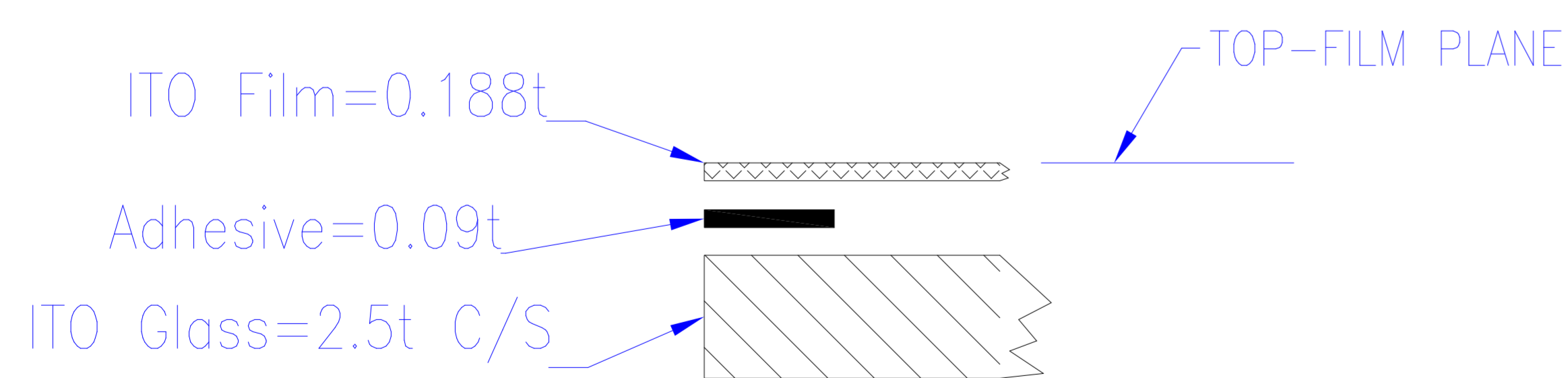
DETAIL A
