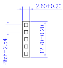
HOUSING
