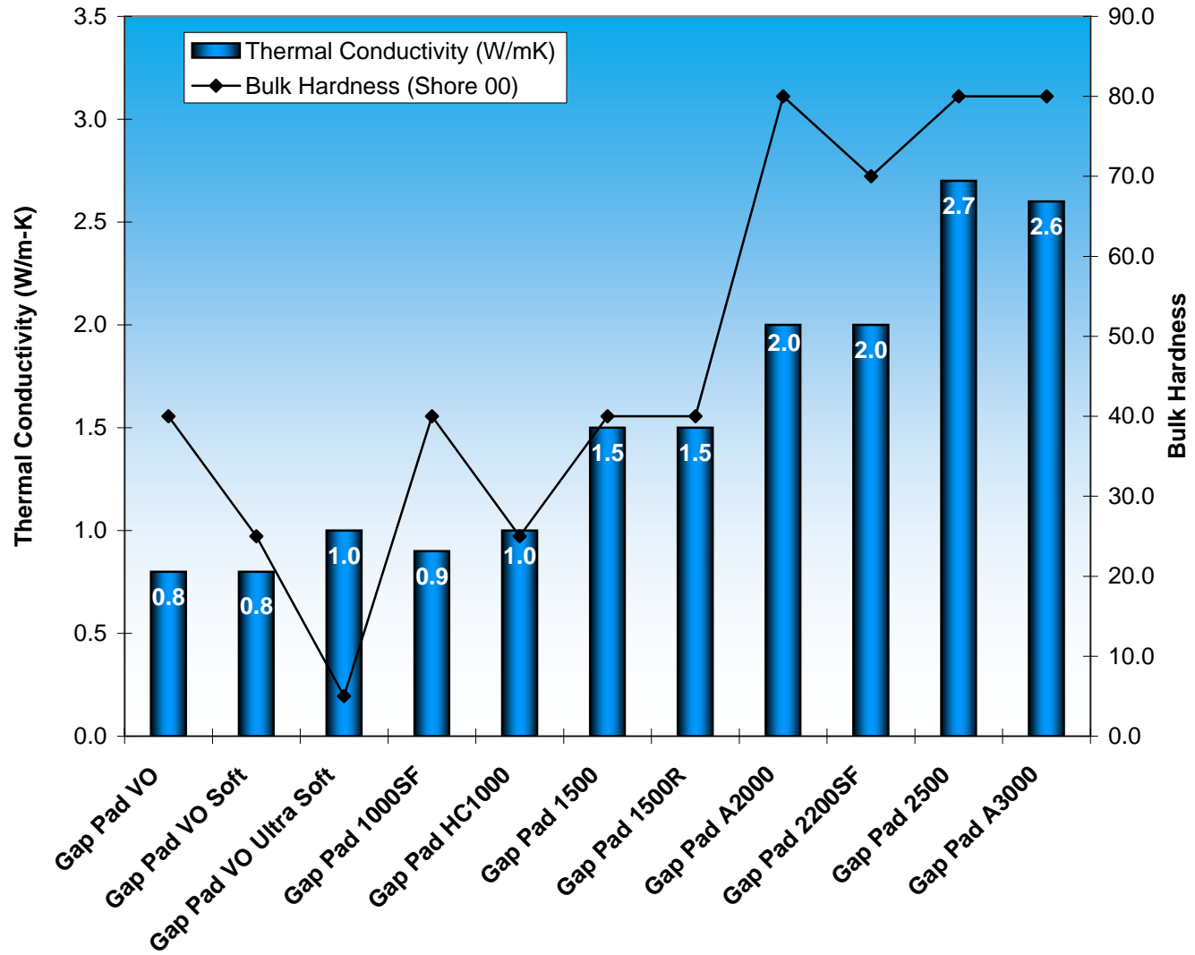
Gap Pad Thermal Conductivity vs. Hardness
