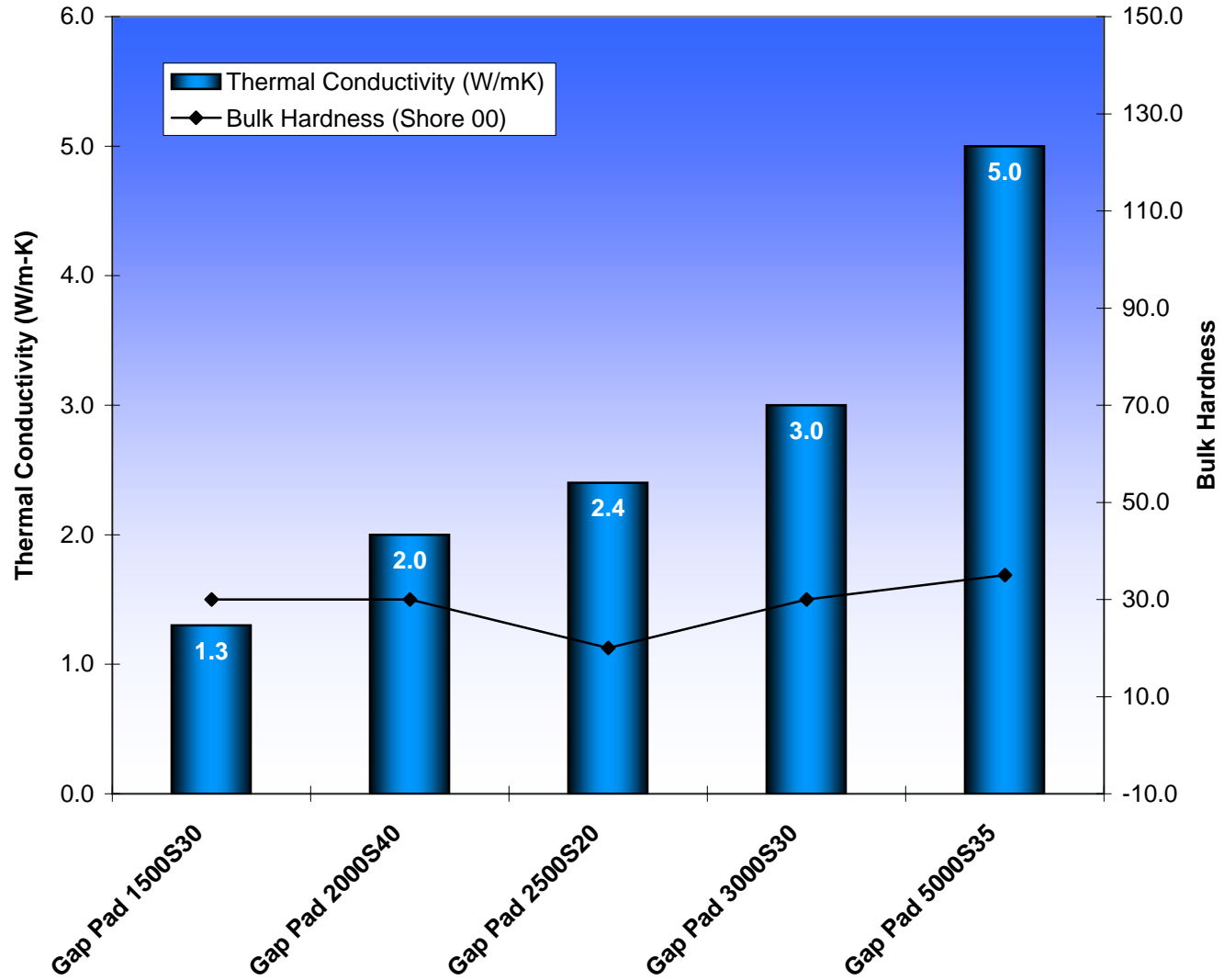
Gap Pad "S Class" Thermal Conductivity vs. Hardness
